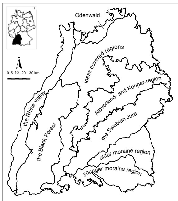
Figure 1. Study region Baden-Wuerttemberg in South West Germany.
